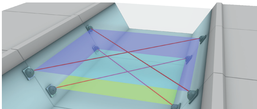
Multi-path Kanalis system with crossed paths in two planes
